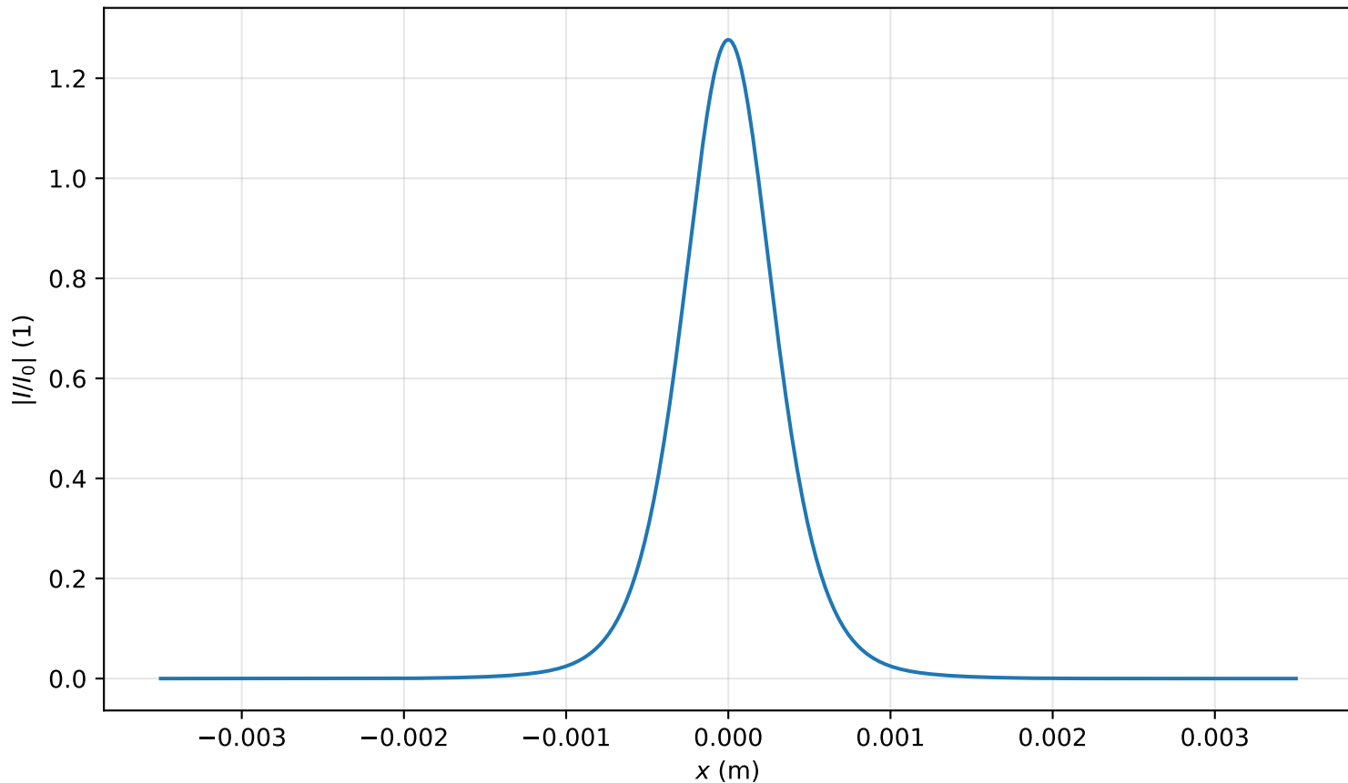
Intensity profile I(x, y = 0, z = 2.229m)/I_0 , P_{in}=0.8P_{cr} , artificial time
